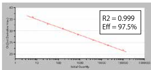
Standard Curve
